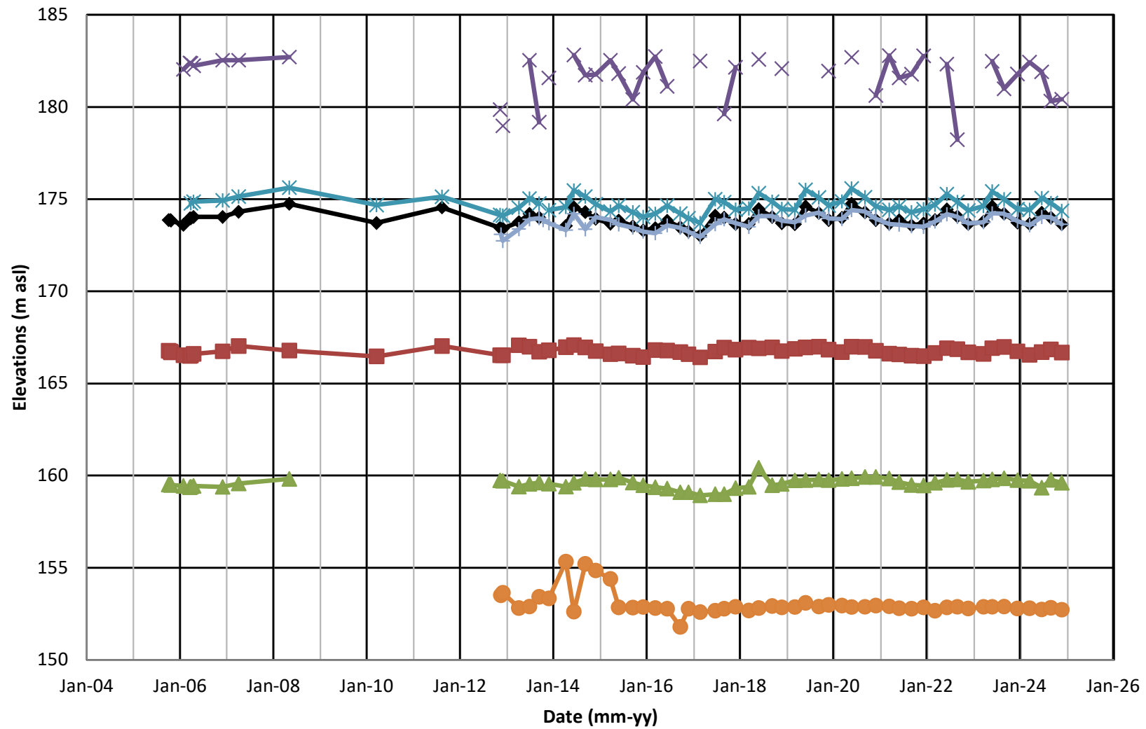
FIGURE B-1 GROUNDWATER ELEVATIONS
